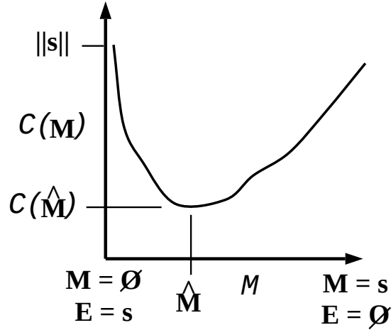
Figure 3 Model optimality. A schematic illustration of the features of the cost function C(M, s) over the model class \mathcal{M} . The topology of the latter is extremely important and is by no means one dimensional. The right portion of the graph is the region of overfitting: so many parameters are used in the model that they begin to directly reflect individual measurements. The left portion of the graph is the region of high apparent randomness: the model captures so little of the data that there is large prediction error.
