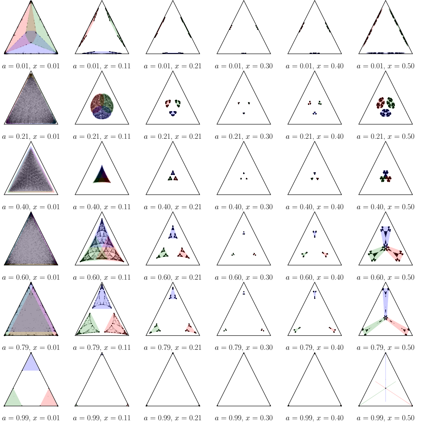
FIG. 5. Mixed-state attractors generated by a 3-state HMC parametrized over \alpha \in [0, 1] and x \in [0, 0.5] . The HMC itself is given in Eq. (16). 10^5 mixed states are plotted for each attractor, with the initial 5 \times 10^4 states thrown away as transients. The ranges of the symbol-labeled maps are color shaded, revealing regions of their image overlap on the attractor. Comparing to Eq. (16), the red, blue, and green regions represent the images of the mapping functions defined by T^\square , T^\triangle , and T^\circ , respectively.
