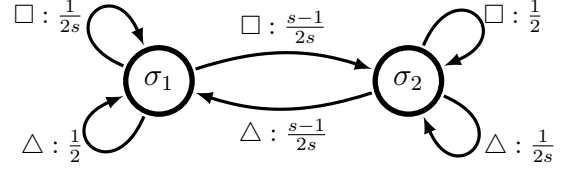
FIG. 1. A hidden Markov chain with two states \mathcal{S} = \{\sigma_1, \sigma_2\} and two emitted symbols \mathcal{A} = \{\square, \triangle\} . It is nonunifilar and parametrized with s \in [1, \infty) . It becomes unifilar in the limit of s \rightarrow \infty .
