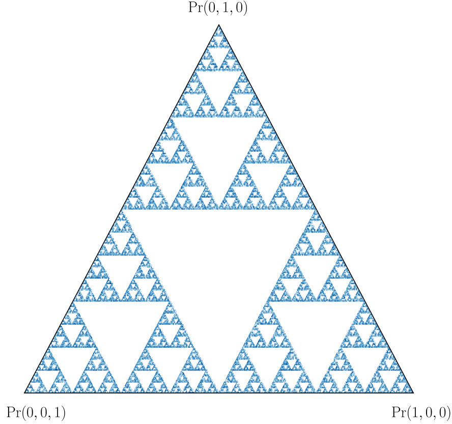
FIG. 8. Attractor of the 3-state, 3-symbol machine specified in Eq. (D1), with s = 2 and a = \frac{1}{6} .
