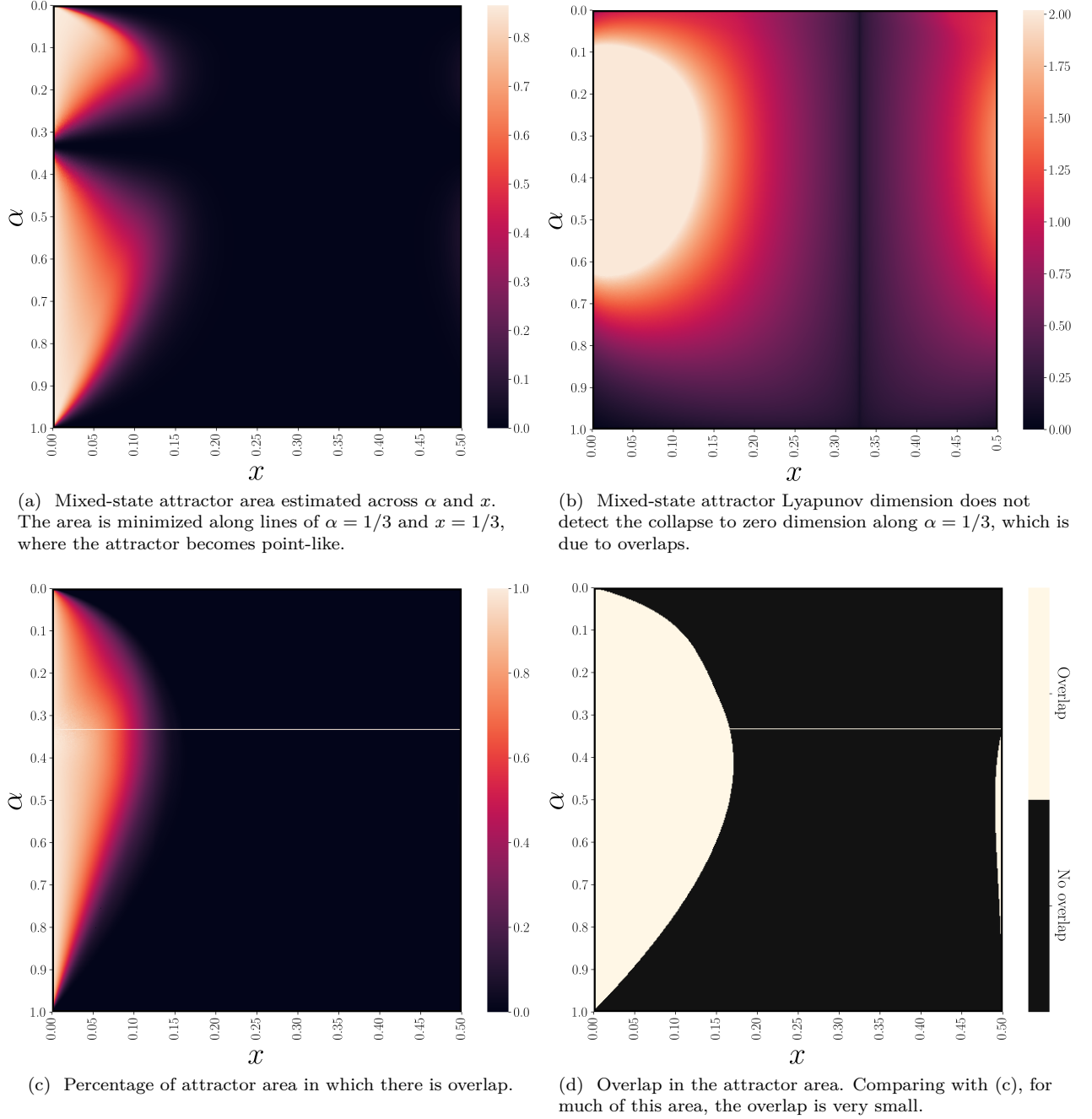
FIG. 6. Attractor area, overlap regions, and Lyapunov dimension of the mixed-state attractors shown in Fig. 5, parametrized by \alpha = [0, 1] and x = [0, 0.5] . The HMC itself is given in Section VI. See Appendix E and Appendix F for a detailed discussion of the production of these plots.
