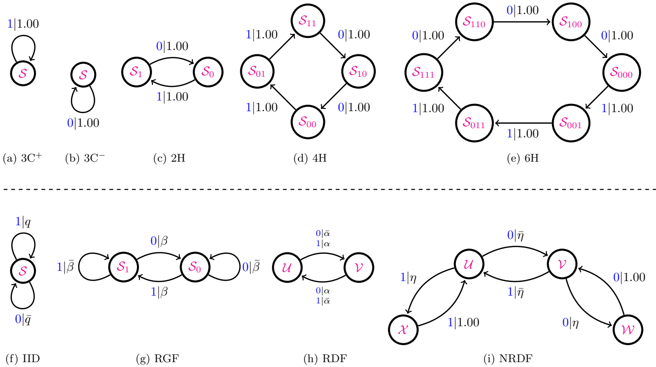
FIG. 1. Nine \varepsilon -machines that represent ordered (a-e; above the dashed line) and disordered (f-i; below the dashed line) material structures. For each the set of output symbols is chosen from \mathcal{A} = \{0, 1\} . The first seven \varepsilon -machines, (a-g), are finite order Markov processes , and the CSs are labeled by \mathcal{S} with subscripts giving the minimum number of previous symbols necessary to uniquely place the process in that CS. In contrast, the last two \varepsilon -machines, (h) and (i), may require an indefinitely long history to place them in a particular CS. These \varepsilon -machines represent strictly sofic processes. The CSs are labeled with the symbols \mathcal{U}, \mathcal{V}, \mathcal{W}, \mathcal{X} . Arcs connecting CSs are labeled s|p , where s is the symbol emitted on transition and p is the probability of a transition. A bar over a transition probability is defined as \bar{p} \equiv 1 - p . (a) 3C^+ crystal structure. (b) 3C^- crystal structure. (c) 2H crystal structure. (d) 4H crystal structure. (e) 6H crystal structure. (f) Independent and identically distributed (IID) process [20, 21]. For q = \bar{q} = 1/2 , the process is maximally random. (g) Random growth fault (RGF) process. For \beta small, we have a randomly twinned 3C structure and, for \beta large, there are random growth faults in the 2H structure. (h) Random deformation fault (RDF) process. For \alpha small, we have random deformation faulting in 2H. (i) Nonrandom deformation fault (NRDF) process. For \eta small, this is nonrandom faulting in 2H; for \eta large, this is a nonrandomly twinned 3C structure.
